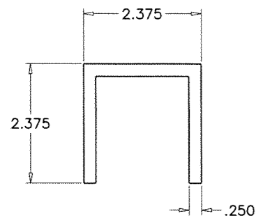
1 TOP/SIDE CHANNEL
