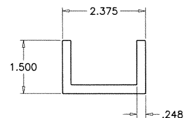
2 BOTTOM CHANNEL
