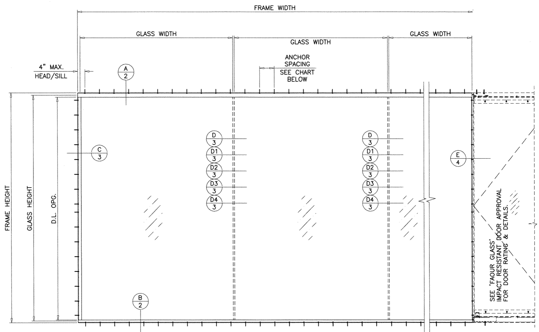
TYPICAL ELEVATIONS
